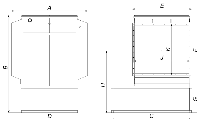
Dimensions of filters CF
