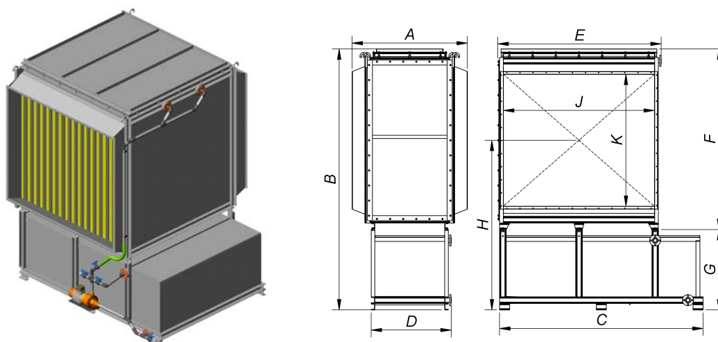
Dimensions of filters of type IEF.
