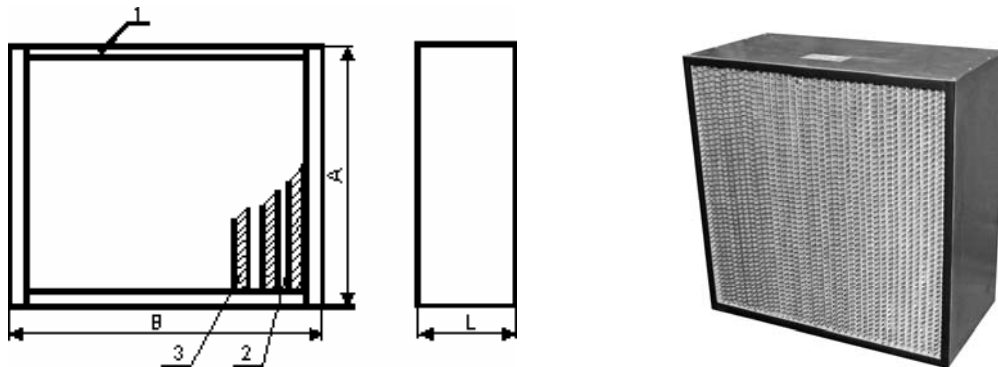
Fig. 1. Scheme of filter CPF.
