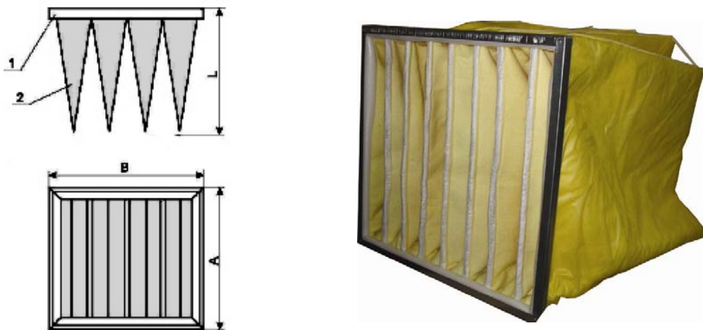
Fig. 1 Scheme of filter of type IPF
