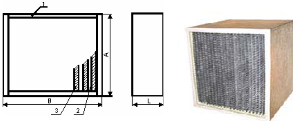
Fig. 1. Scheme of filter CCF.
